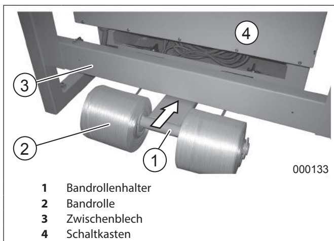
Abb. 5 Bandrollen
