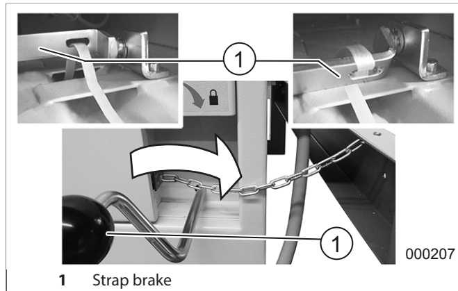
fig. 14 Strap brake
